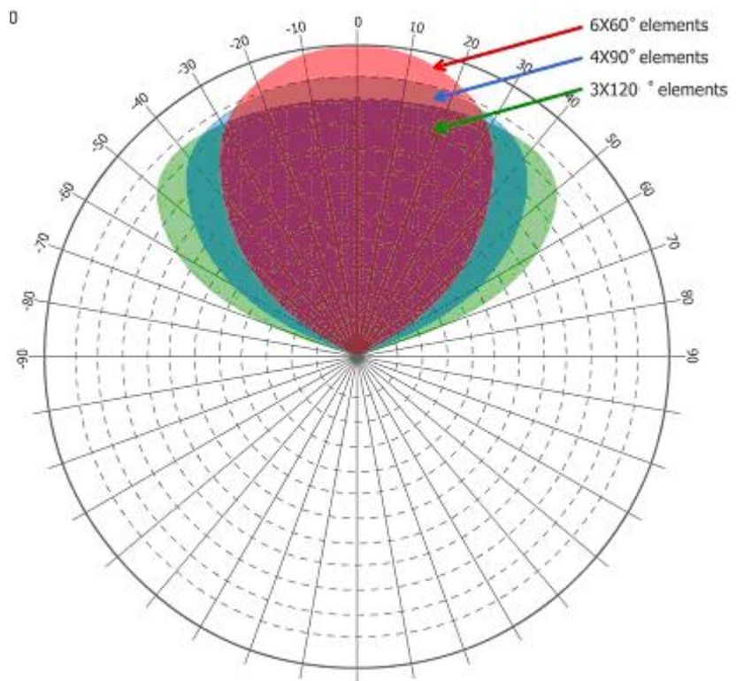
Figure 2. 3, 4 and 6 Elements Array
