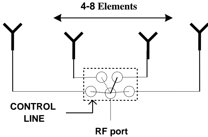
Figure 1. Schematic Diagram of a 4 Element Unit
