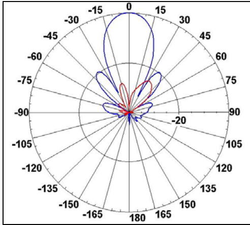
Azimuth Radiation Pattern Midband Freq. 2.6 GHz
