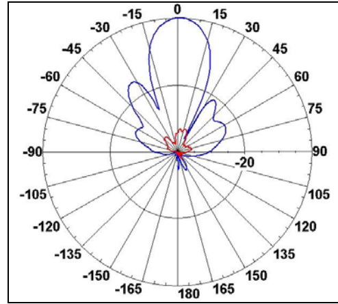
Elevation Radiation Pattern Midband Freq. 2.6 GHz
