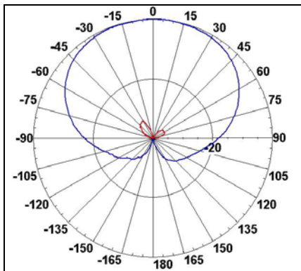
Azimuth Radiation Pattern Midband Freq. 2.5 GHz
