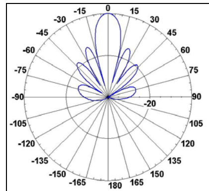
Elevation Radiation Pattern Midband Freq. 2.5 GHz
