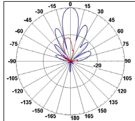
Elevation Radiation Pattern Midband Freq. 2.5 GHz
