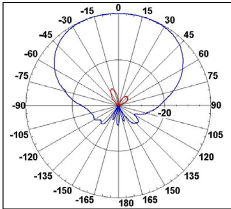
Azimuth Radiation Pattern Midband Freq. 2.5 GHz
